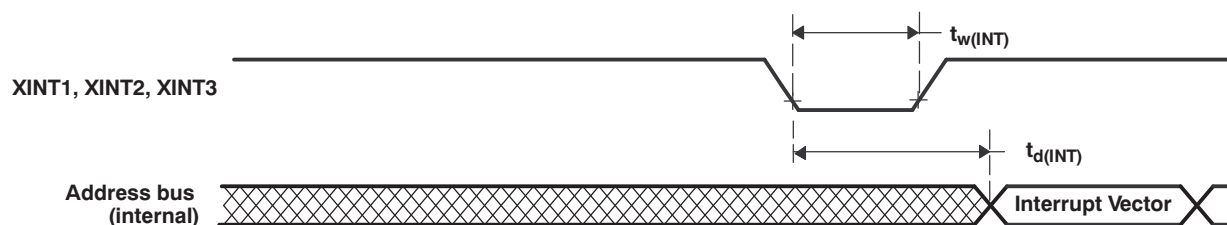
Figure 6-15. External Interrupt Timing
