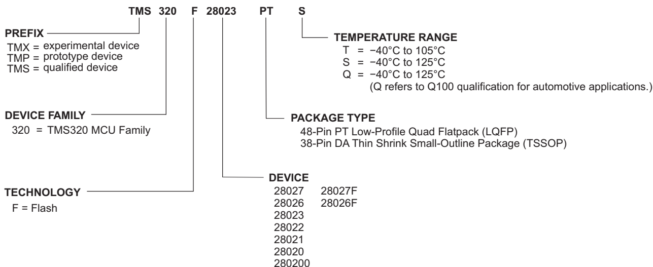
Figure 8-1. Device Nomenclature
